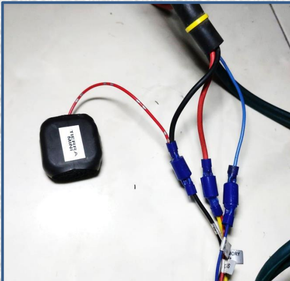
Installation of Tierra Mini in Head Unit
